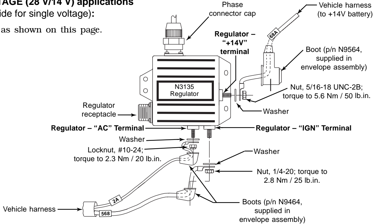
Figure 1a – N3135 Regulator Dual Voltage Wiring Connections
