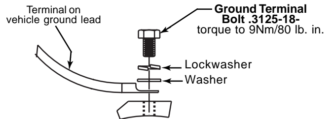
Figure 1b – Ground Terminal Connections
