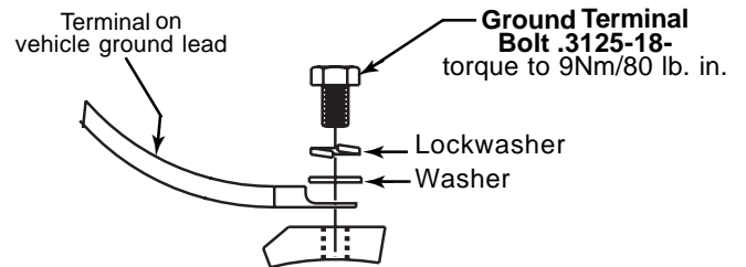
Figure 1c – Ground Terminal Connections
