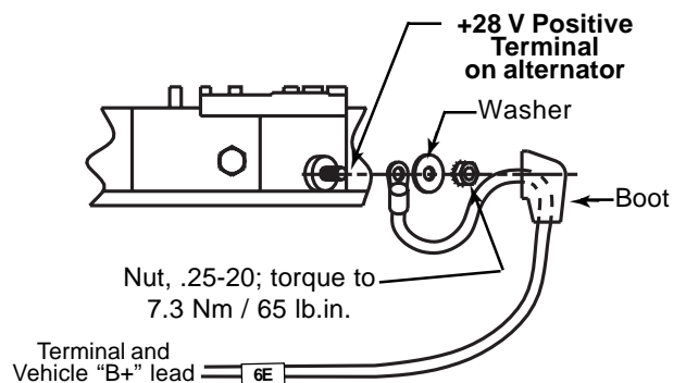
Figure 1c – Positive Terminal Connections
