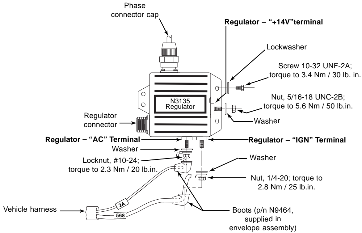
Figure 1a – N3135 Regulator Single Voltage Wiring Connections
