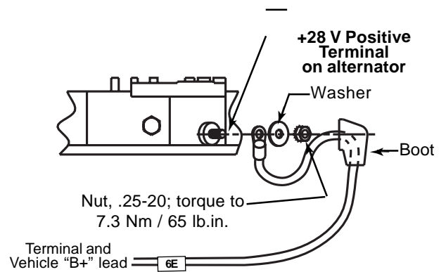
Figure 1b – Positive Terminal Connections
