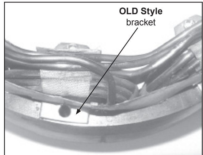
Figure 2: "OLD" Style Bracket on Stator Assembly
