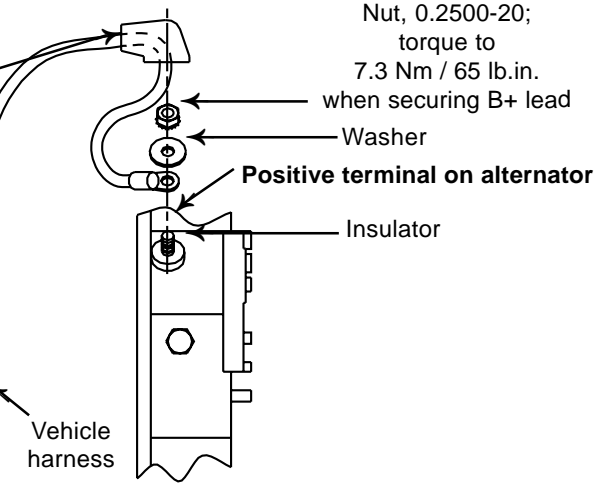
Figure 1c - Positive Terminal Connections
