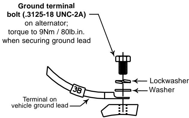
Figure 1b - Ground Terminal Connections
