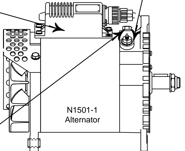
Figure 1 - N1501-1 Alternator
