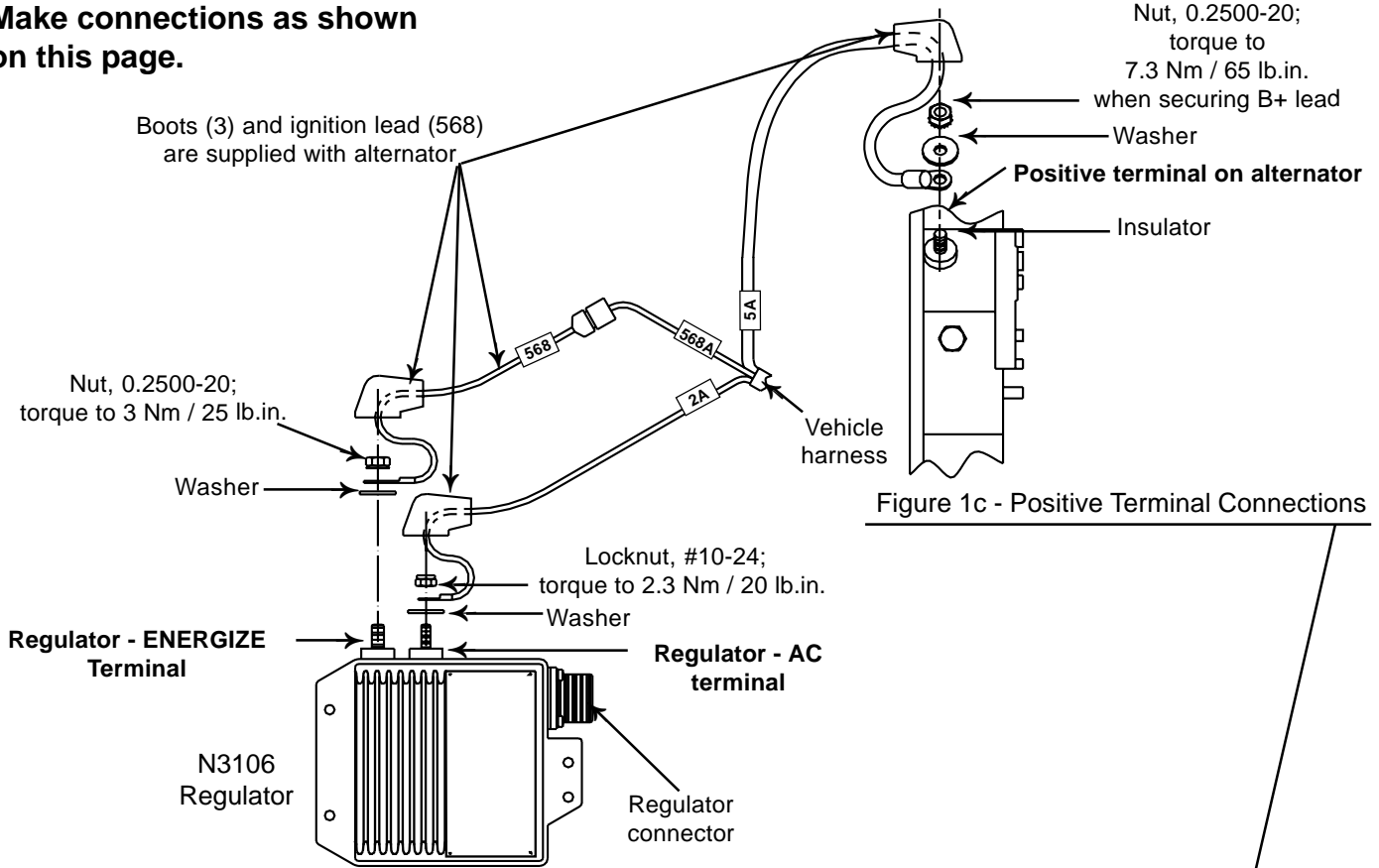
Figure 1a - N3106 Regulator Wiring Connections
