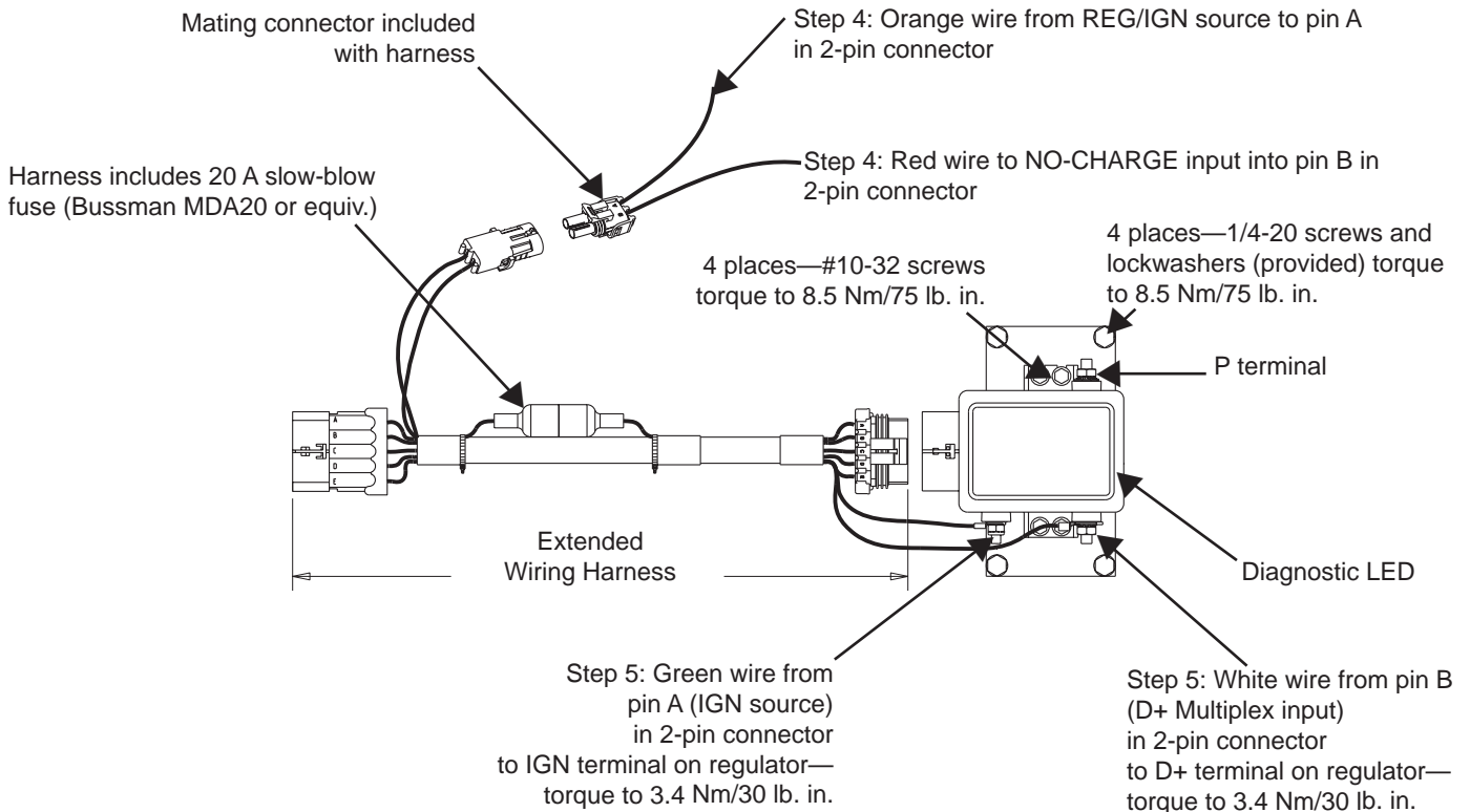
Figure 2 – Remote-Mounted Commercial Regulator with Extended Alternator Wiring Harness
