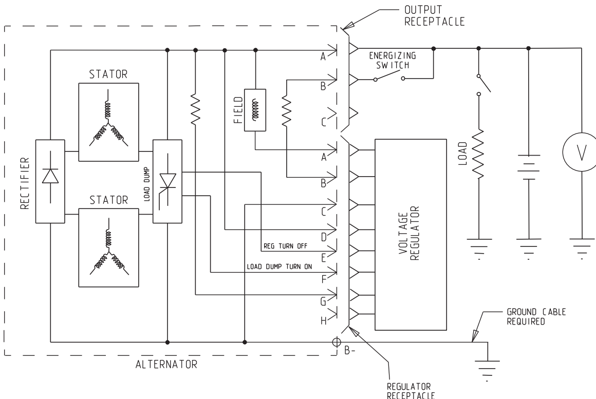
Figure 3 — NI326-I Alternator with N3007 Regulator Wiring Diagram
