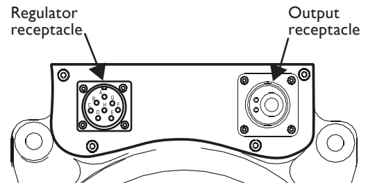
Figure 1 — NI326-I Control Assembly
