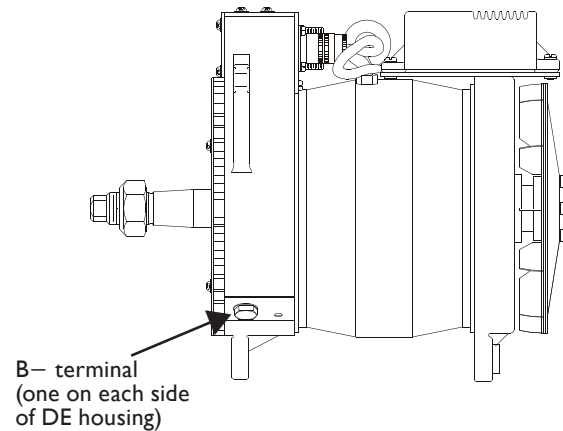
Figure 2 — NI326-I Alternator Terminals (N3007 Regulator Attached to Alternator)
