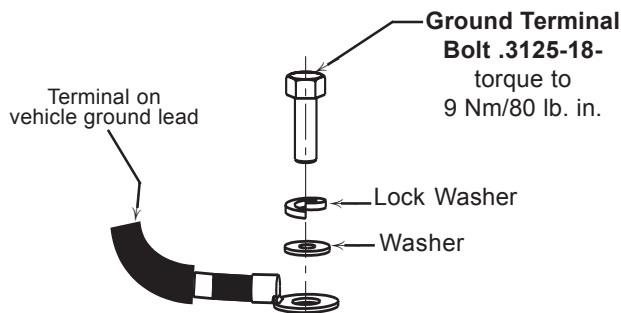
Figure 3b – Ground Terminal Connections
