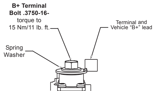
Figure 3c – Positive Terminal Connections
