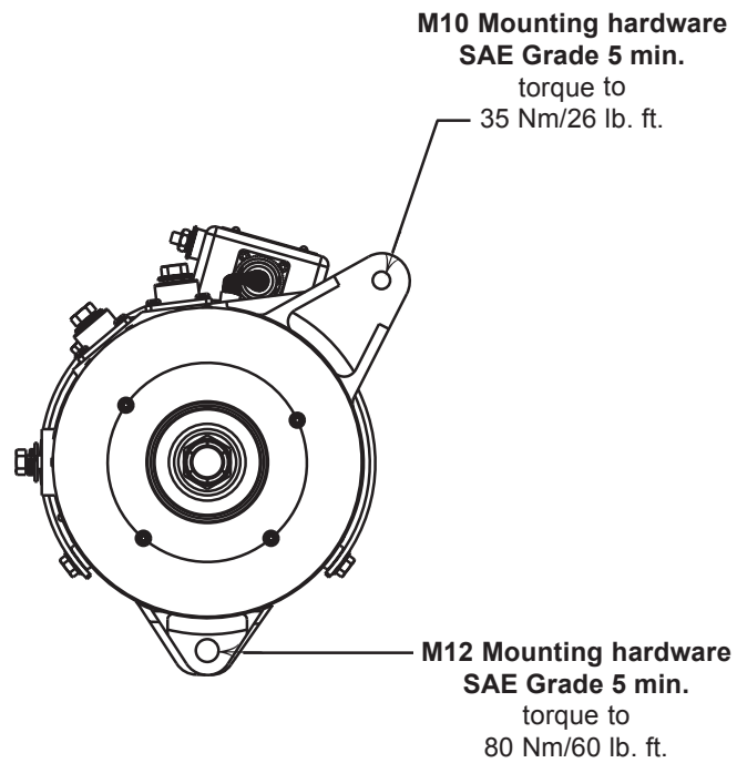
Figure 1 – N1511-1 Alternator Mounting
