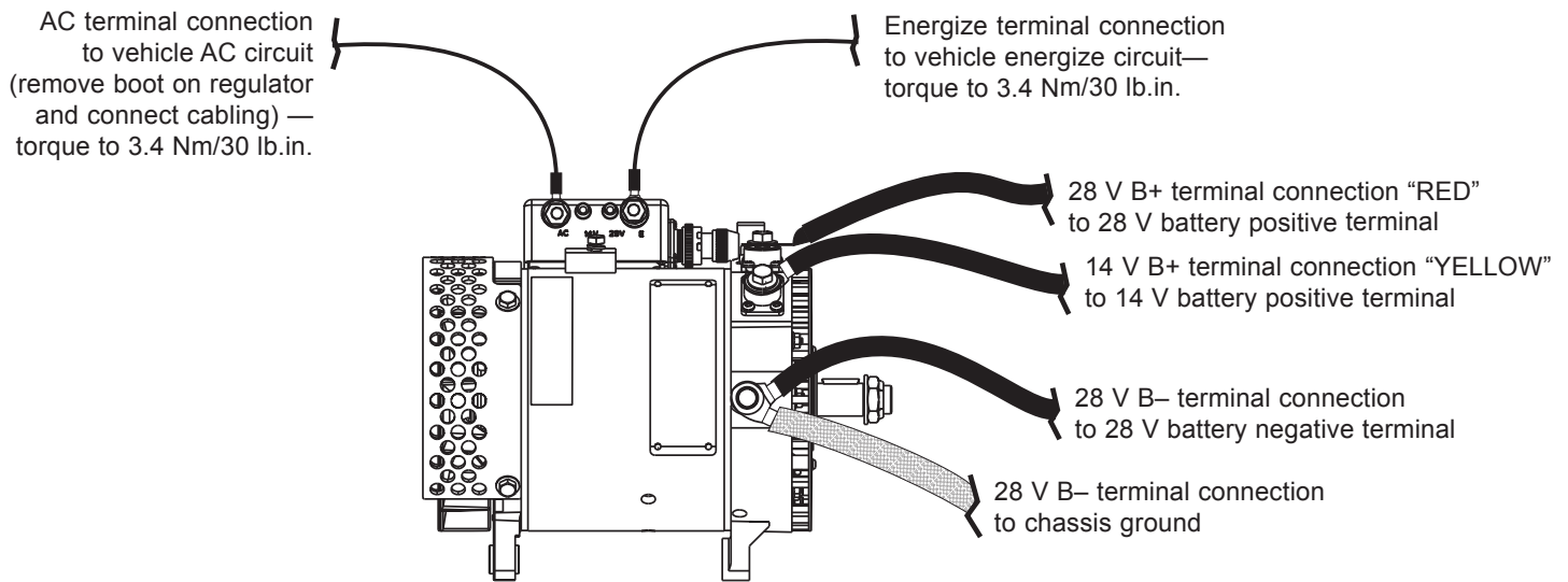
Figure 3a – N1511-1 Wiring Connections
