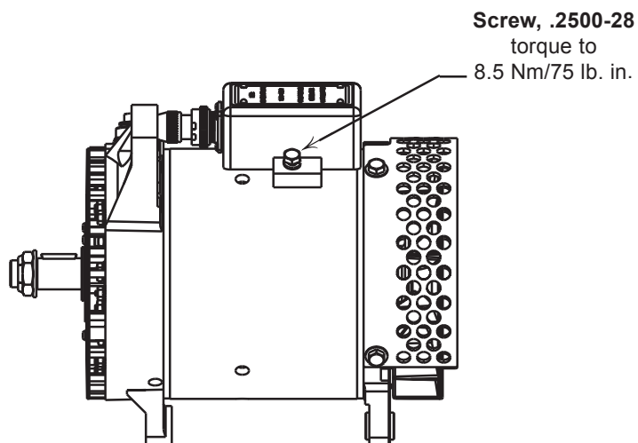
Figure 2 – N1511-1 Regulator Mounting
