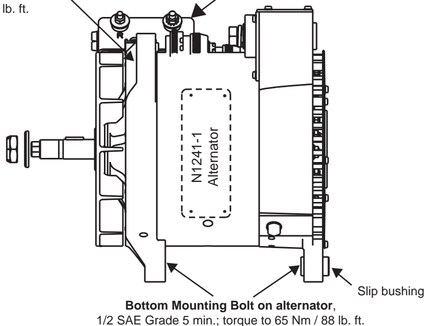
Figure 1– N1241-1 Alternator
