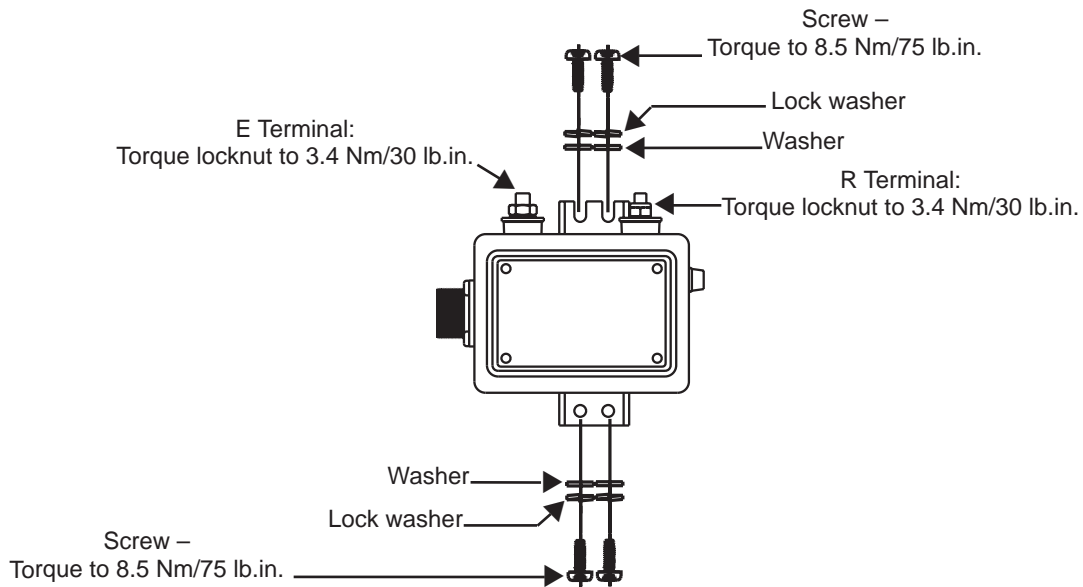
Figure 1a – N3208 Regulator Wiring Connections
