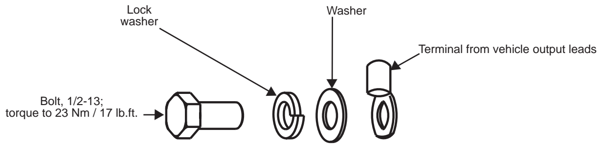
Figure 1b – 28 V or 14 V B+ Terminal Stacking Order
