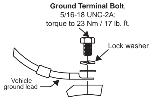
Figure 1c – Ground Terminal Stacking Order
