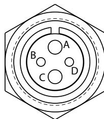
Figure 5: Alternator Harness Socket Connections
