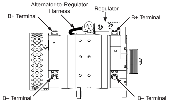
Figure 1: N1604 Alternator
