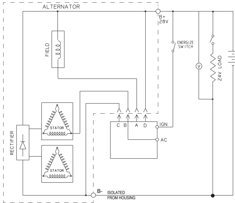
Figure 3: N1604 Alternator Wiring Diagram
